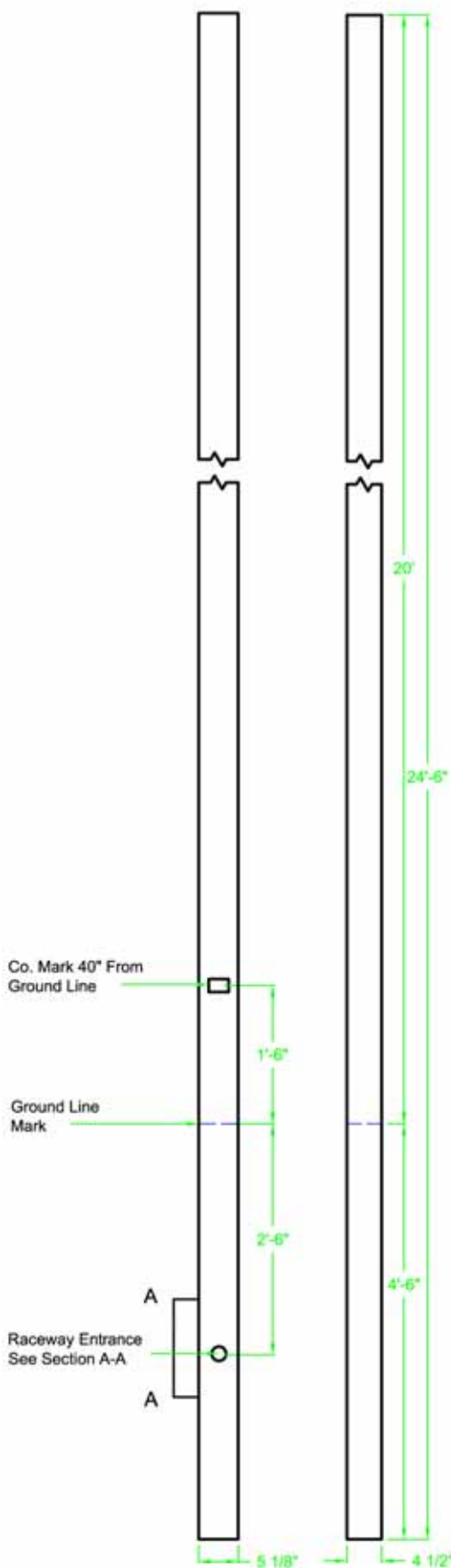
Pole Details
