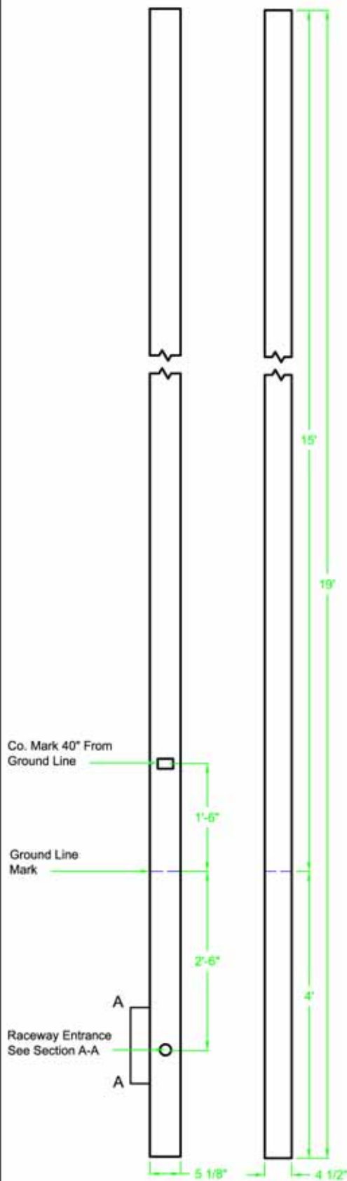
Pole Details
